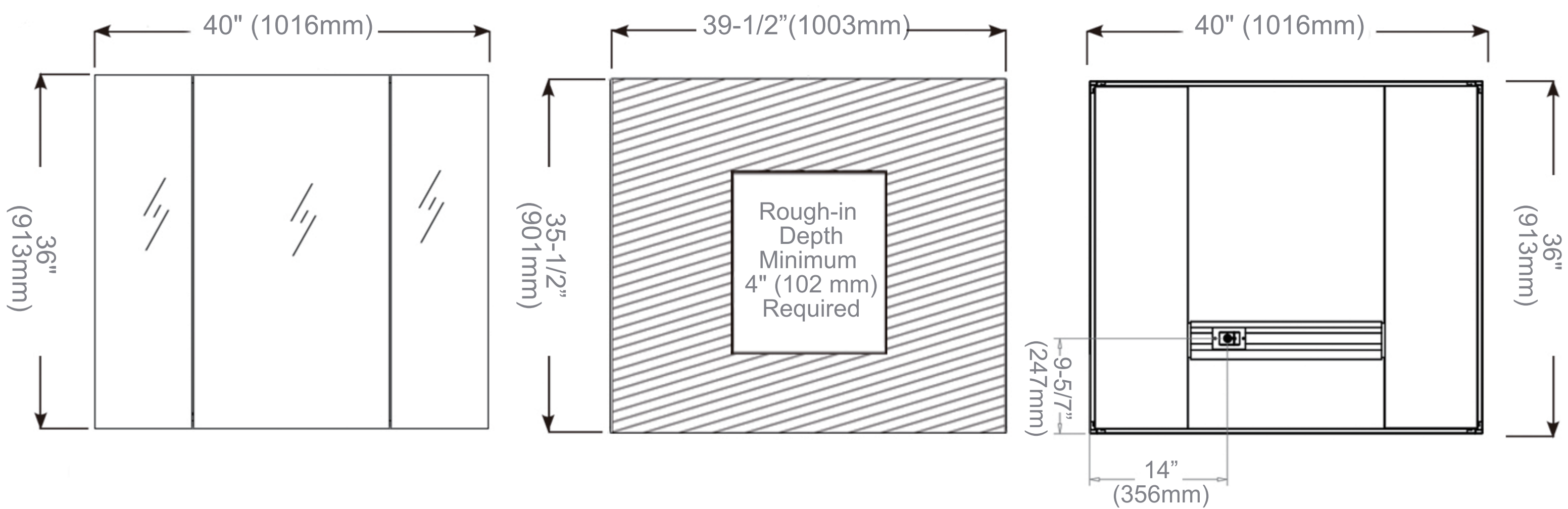
Cabinet Dimensions
